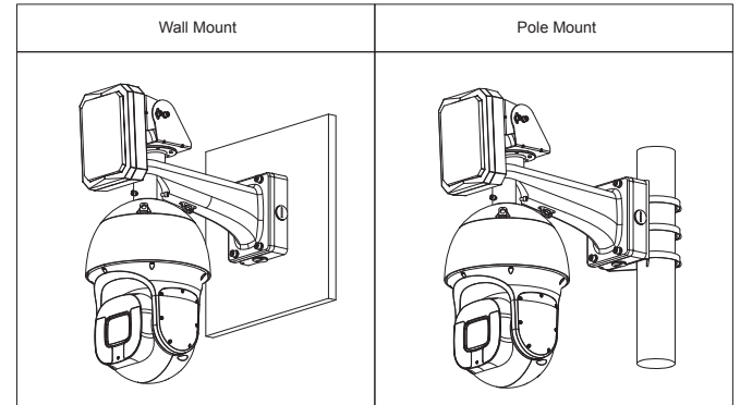
PFA150 Pole Mount Bracket
