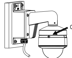
C: Fastening screw on dome
